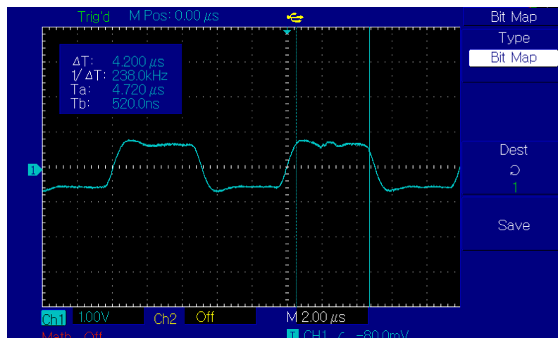
Effect of capacitance fig. 13.2
